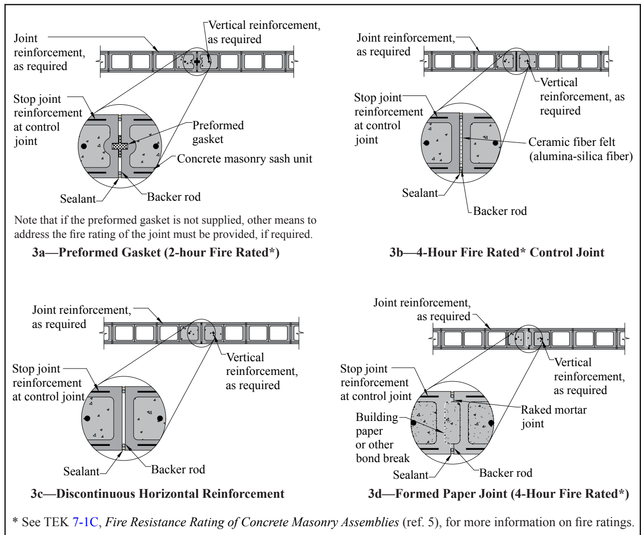
Figure 3—Typical Control Joint Details (continued on next page)
